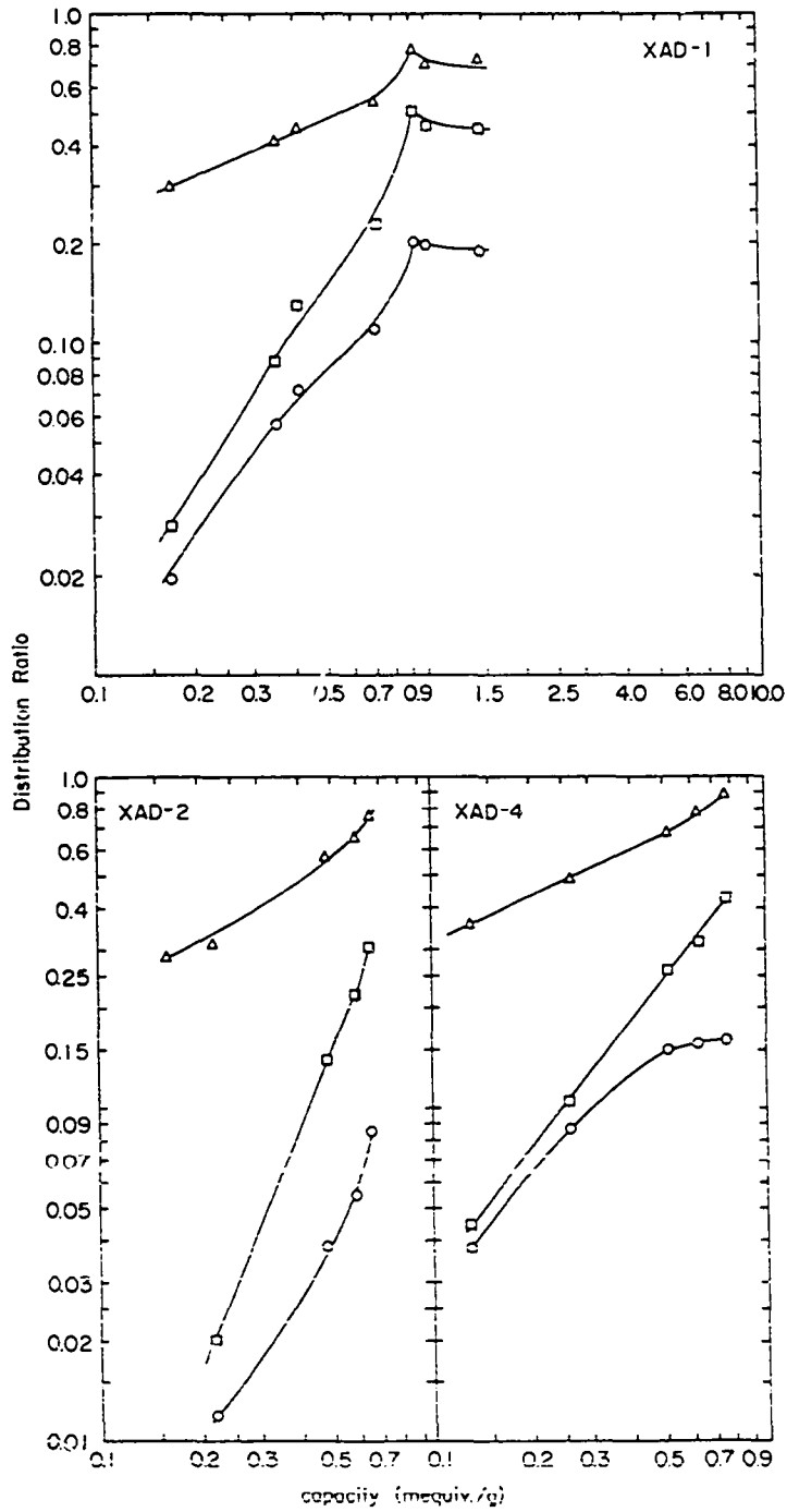
Figure 1. Distribution ratios of anions for resins of different capacity; Eluent: 4 \times 10^{-4} M sodium bicarbonate and 3 \times 10^{-3} M sodium carbonate Δ, acetate; □, iodate; O, fluoride
