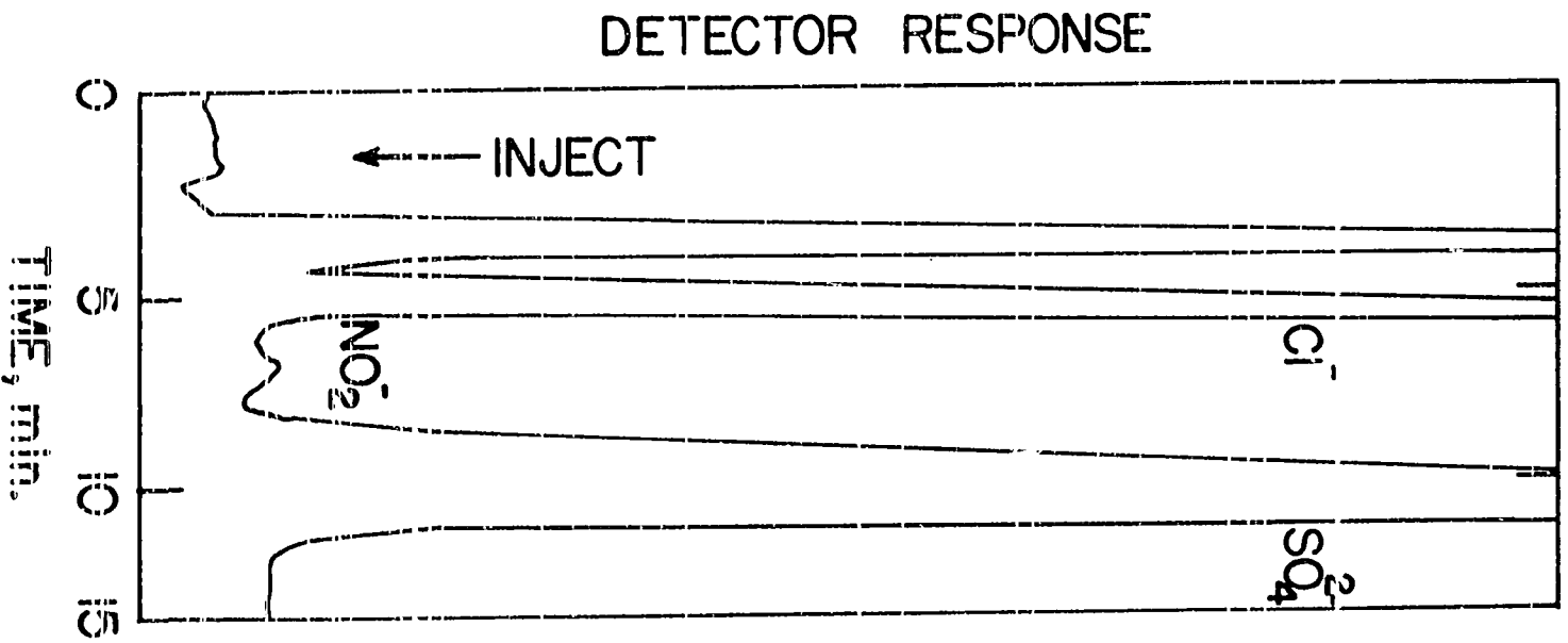
Figure 10. Separation of 0.37 ppm nitrite from chloride and sulfate in ISU tap water; Resin: Vydac SC anion exchange; Eluent: 5 \times 10^{-4} M KHP, pH = 6.0
