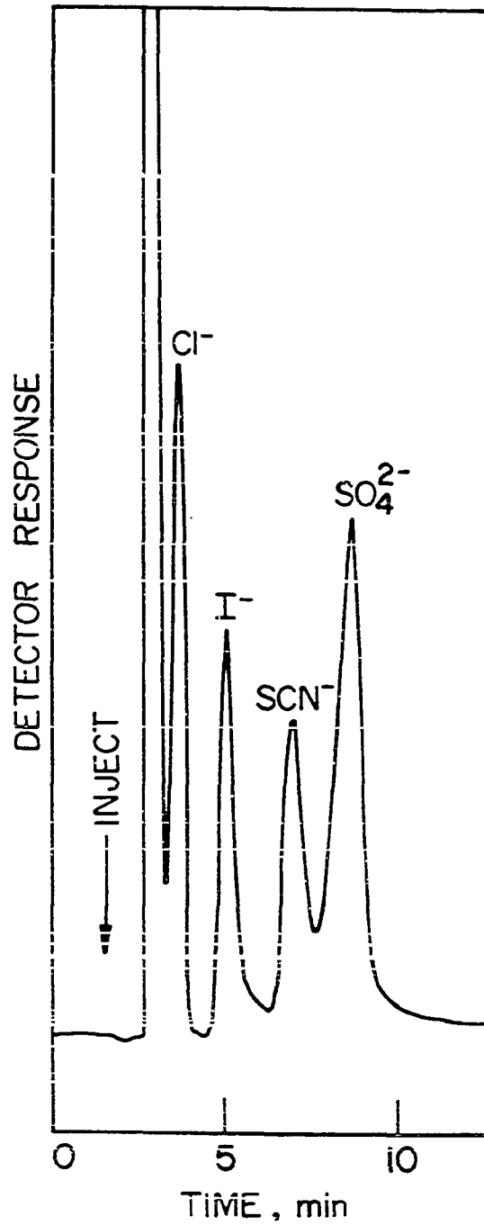
Figure 6. Separation of 7.7 ppm chloride, 29.5 ppm iodide, 28.6 ppm thiocyanate and 16.5 ppm sulfate; Resin: XAD-1 0.007 mequiv./g; Eluent: 1 \times 10^{-4} M KHP, pH = 7.1
